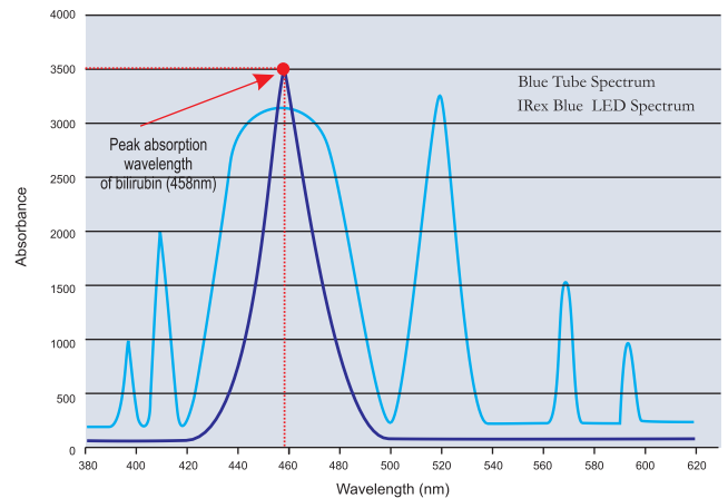
Comparison of Blue LED Spectrum with Blue Tube Spectrum (Spectrum analysed by International School of Photonics, CUSAT)
